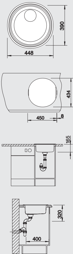
Bowl depth: 165mm
