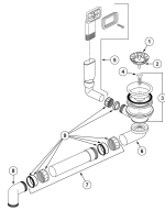
Spare waste set BLS00227384
