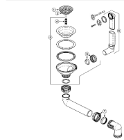
Spare waste set BLS00220468
