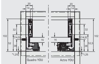
270mm Quadro YOU runner, silent (30kg) HE9256854 (L) HE9256855 (R)
