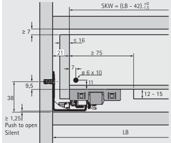
Push-To-Open silent operating system HE9257892
